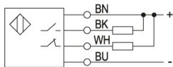
NPN NO+NC
